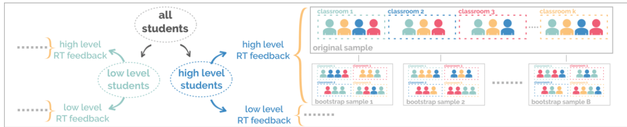
Figure 5. Bootstrap sample generation process used in Algorithm 1. Details are given for the case of high-level students who received high-level feedback, but the exact same process applies to the other three cases.
